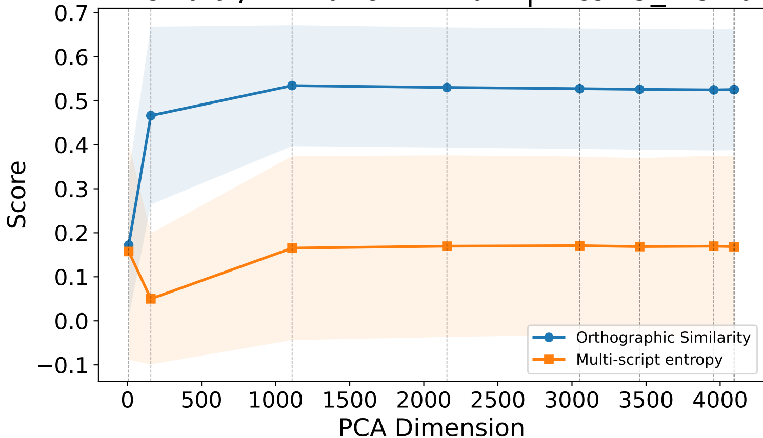
mistralai/Mixtral-8x7B-v0.1 | mcs=5_ms=6
